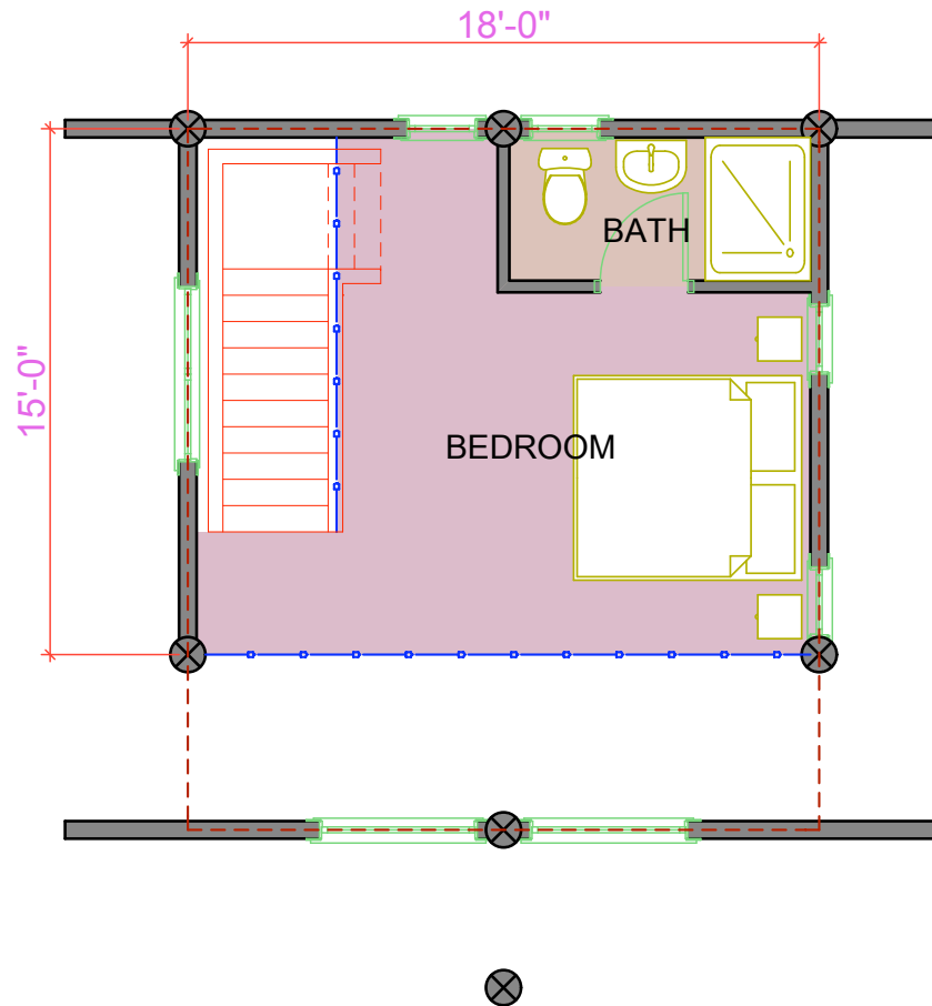
SECOND FLOOR PLAN AREA: 208 SQ. FT.
