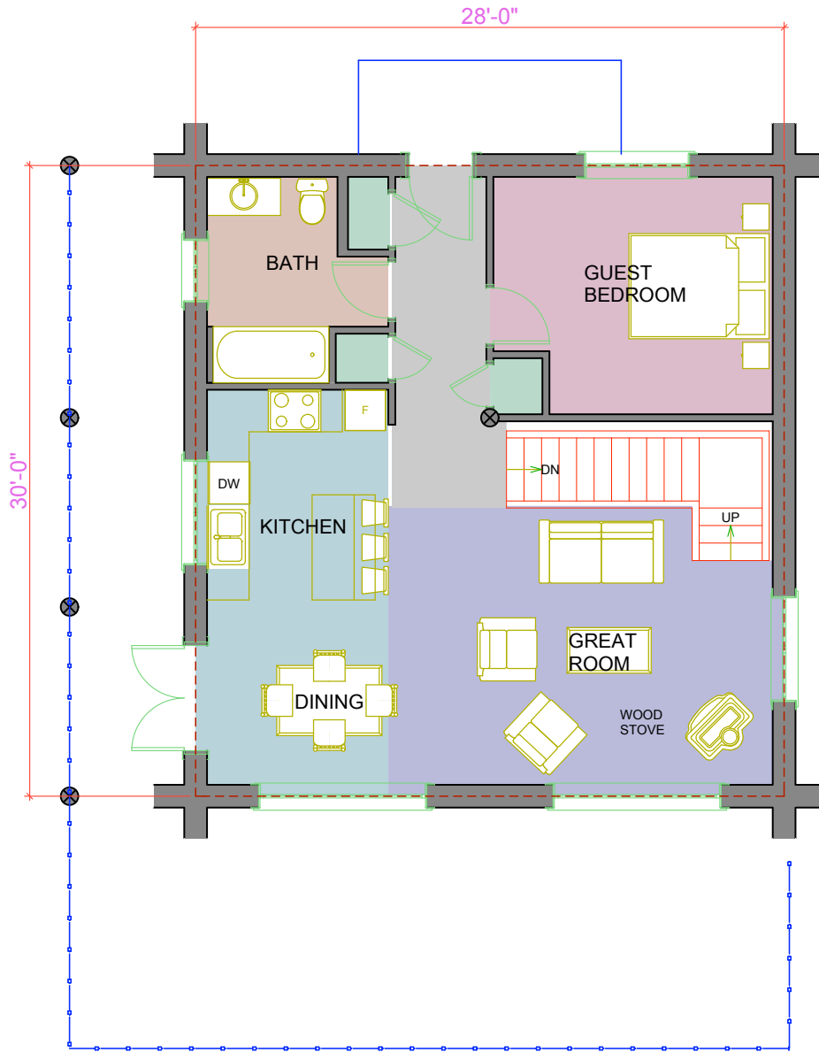
FIRST FLOOR PLAN AREA: 870 SQ.FT.
