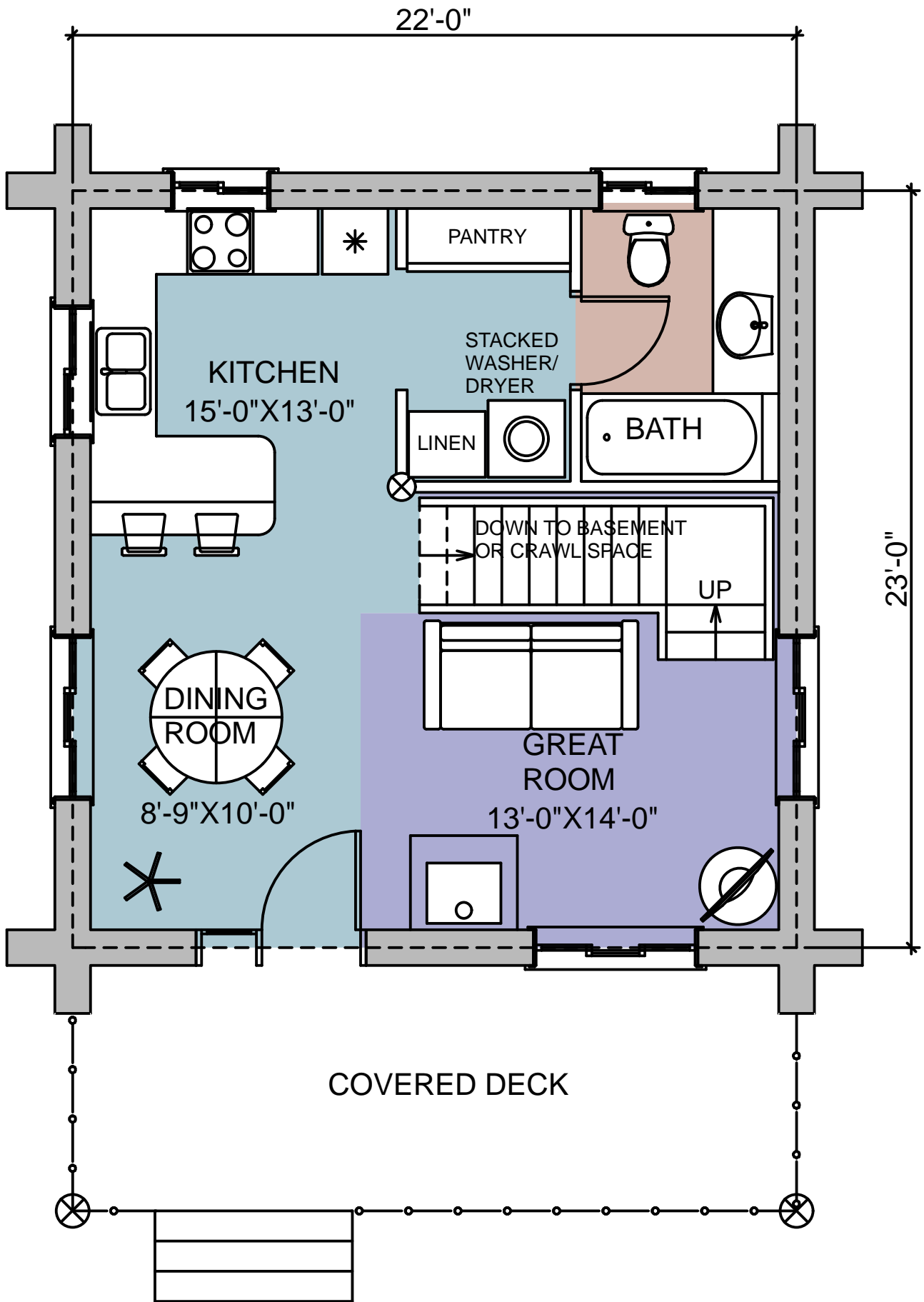
FIRST FLOOR PLAN AREA: 506 SQ.FT.
